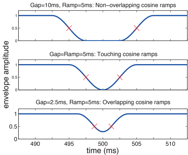
Figure 5.1 Examples of ramped envelopes used to create the gapped stimuli. The gap size was defined as the interval between the midpoints of the on- and offset ramp as shown by the markers. The envelope did not reach zero for gap sizes smaller than the ramp duration due to overlap of the on- and offset ramps (e.g. in lowest panel).
